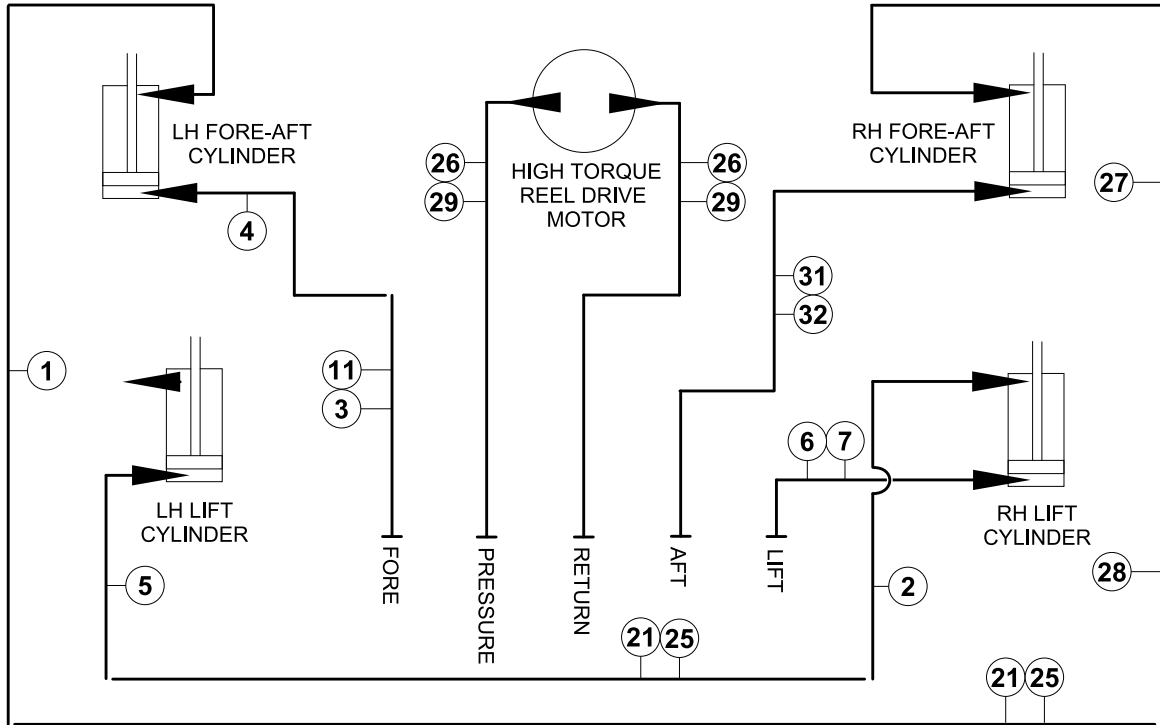
HYDRAULIC SCHEMATIC: 15' and 20' SINGLE REEL RIGID HEADER
