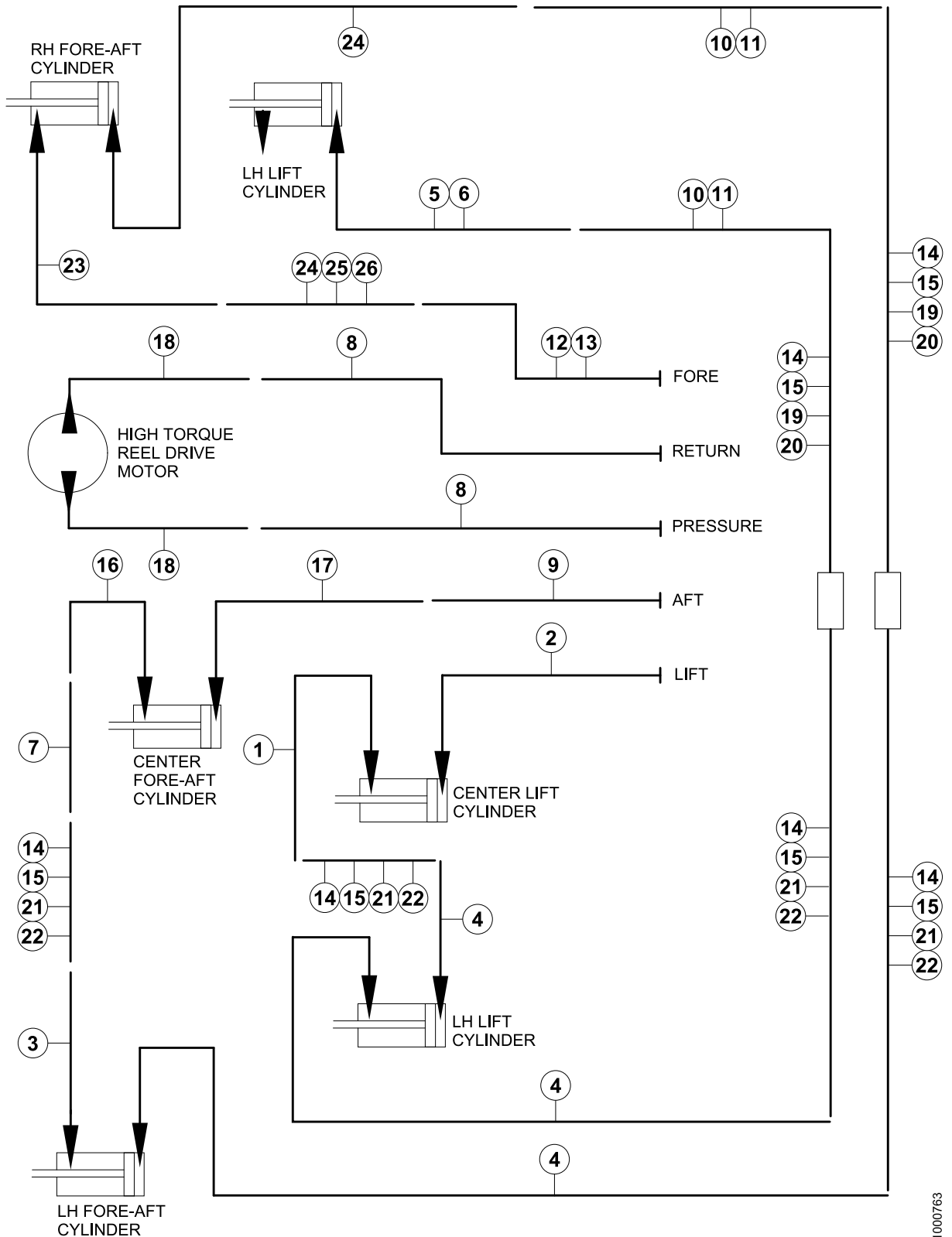
HYDRAULIC SCHEMATIC: 30' - 45' DUAL REEL RIGID HEADER
