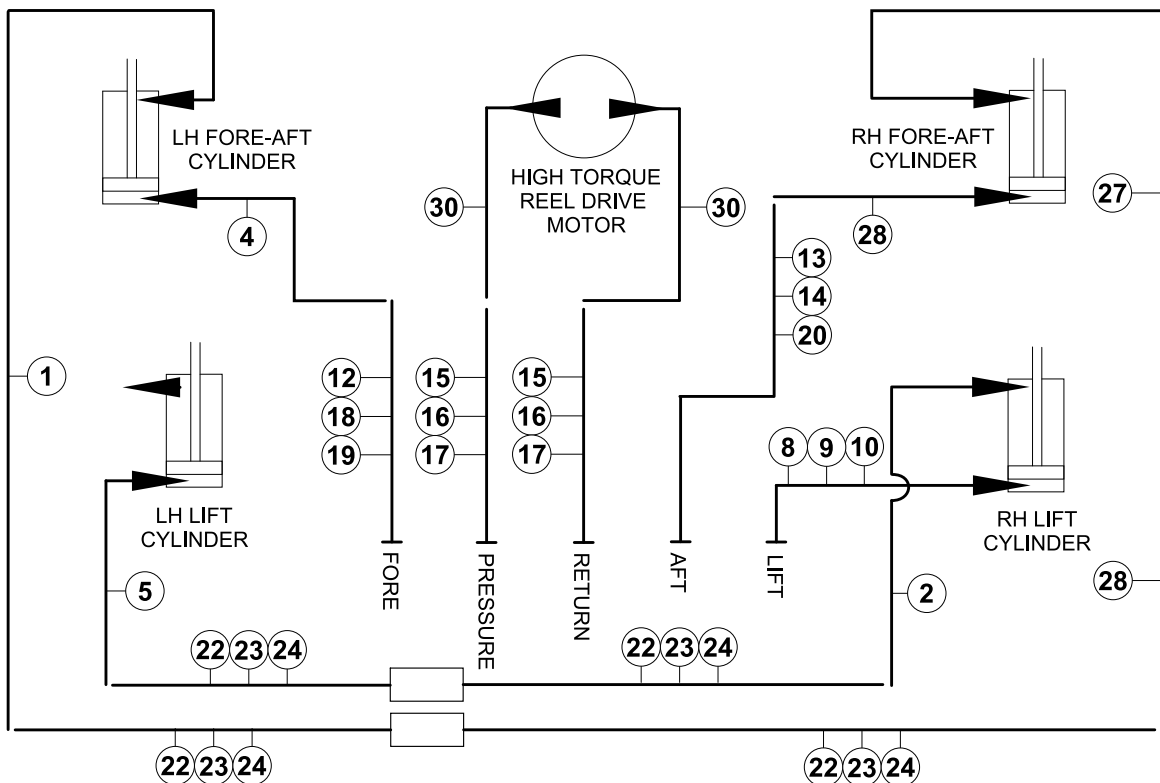
HYDRAULIC SCHEMATIC: 25' - 35' SINGLE REEL RIGID HEADER
