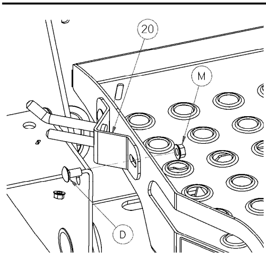
LH PLATFORM REMOVED FOR CLARITY
