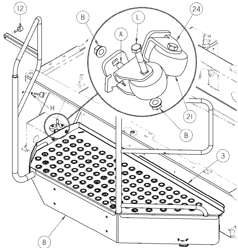
LH PLATFORM
