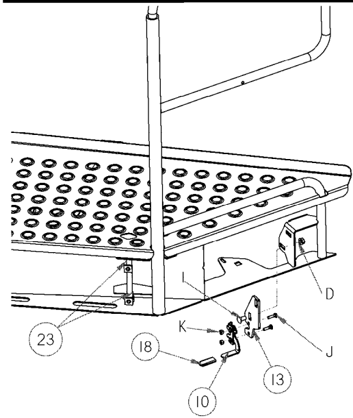
LH PLATFORM
